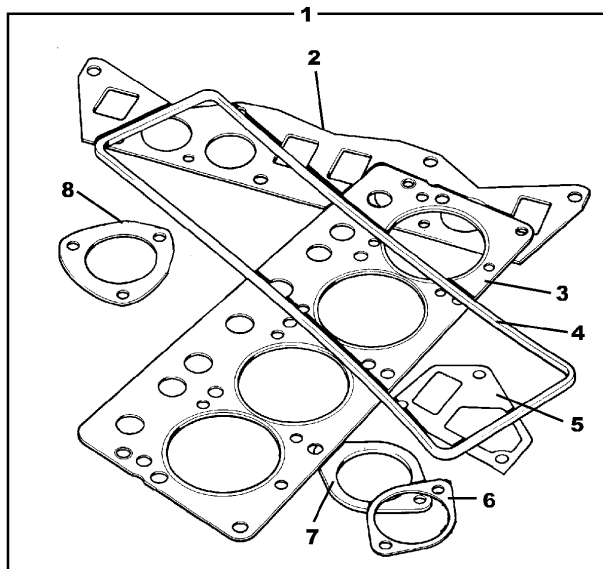
Engine Gaskets
